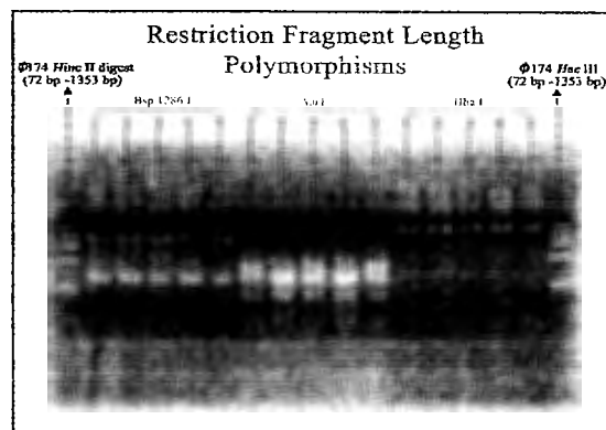
Figure 2b. Photograph RFLP analysis of the PCR product
