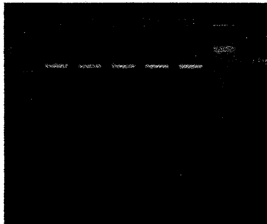
Figure 2a. Photograph PCR product of the 16S ribosomal RNA gene from DNA mitochondria of the tropical anguillid eels
